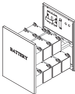
14pcs Batteries 33AH 196 × 131 × 156 (L × W × H)
