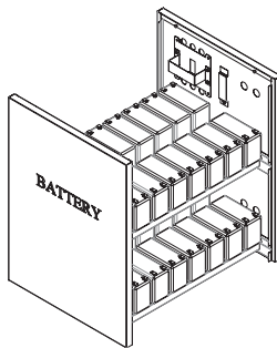
32pcs Batteries 6AH/7AH/9AH 151 × 65 × 100 (L × W × H)
