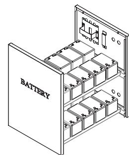
20pcs Batteries 12AH 151 × 98 × 100 (L × W × H)
