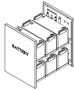
6pcs Batteries 100AH/120AH 407 × 174 × 236 (L × W × H)
