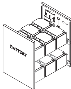
12pcs Batteries 38AH/45AH 198 × 166 × 170 (L × W × H)
