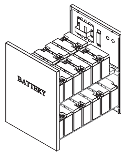
26pcs Batteries 15AH/20AH/22AH 181 × 77 × 167 (L × W × H)
